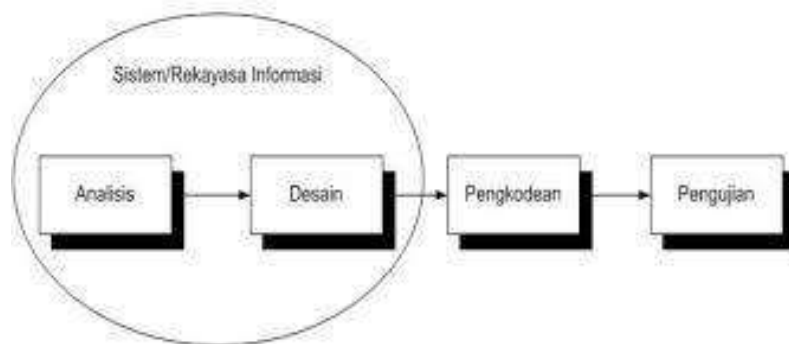
Gambar 3. 1. Metode Waterfall
