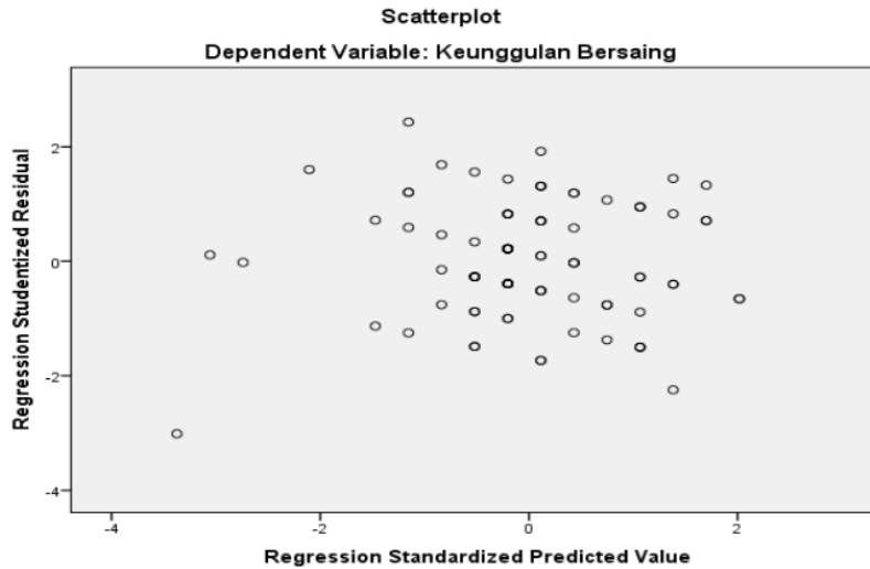
Gambar 1. Scatter Plot
