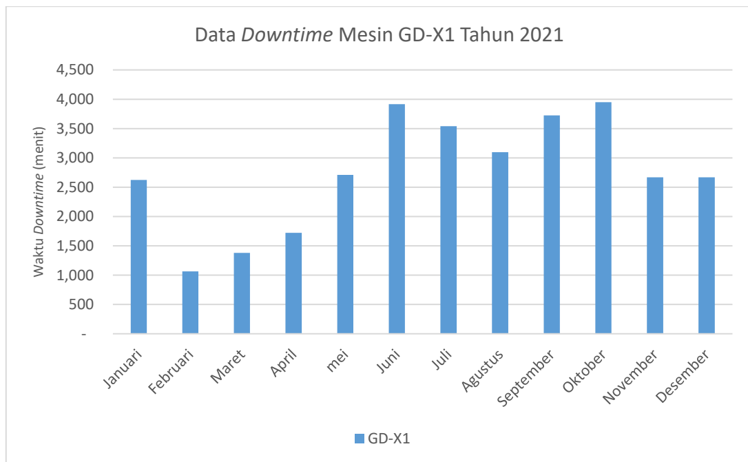
Gambar 1.2 Data Downtime Mesin GD-X1
