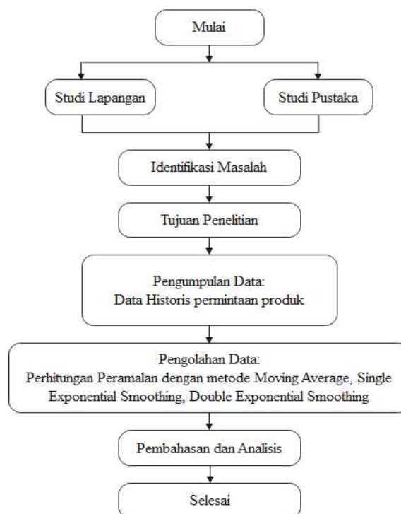
Gambar 3.1 Flow Chart
